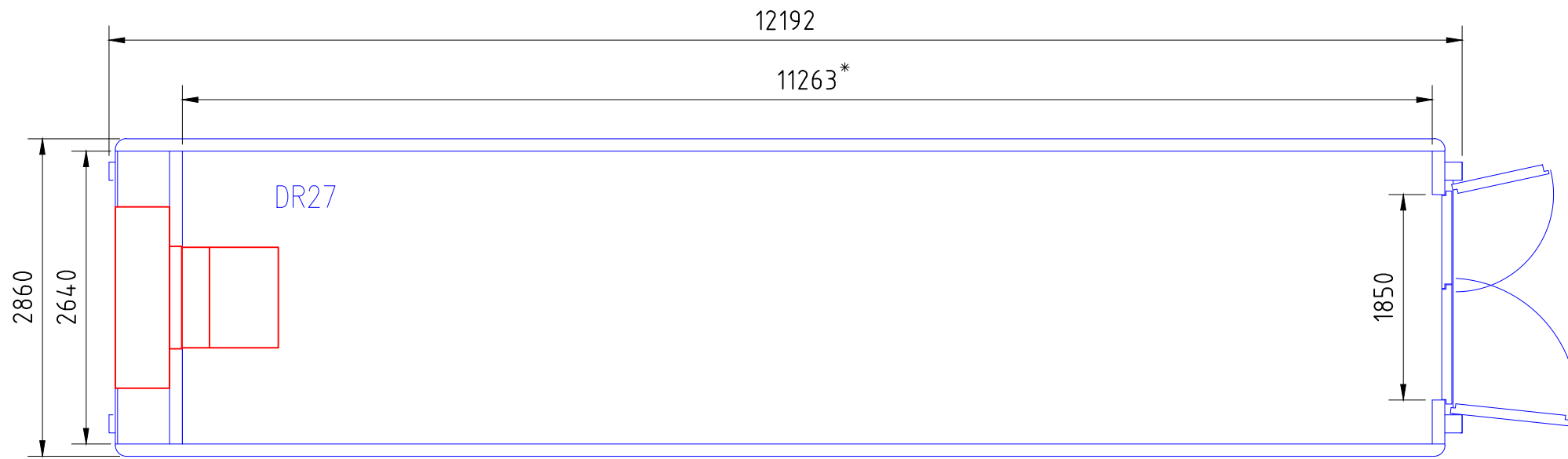
PLAN VIEW
