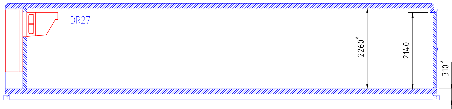
SIDE SECTION
